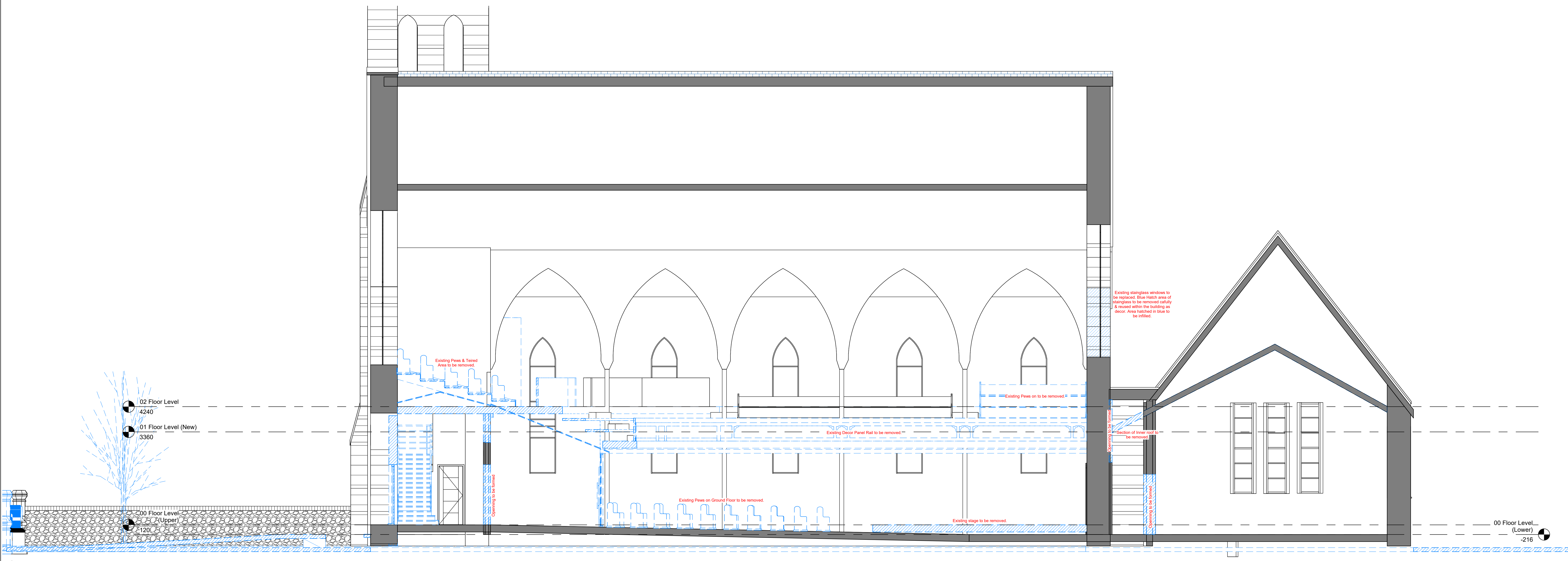
2 Existing Section 03 1:50
